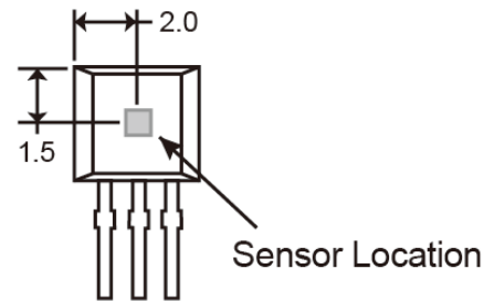
Hall Chip Location (Top View)
