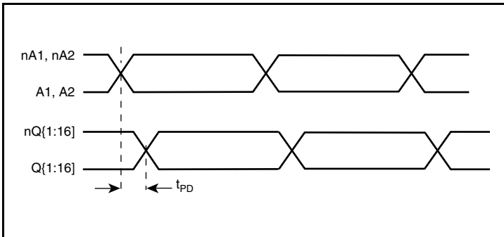
Propagation Delay
