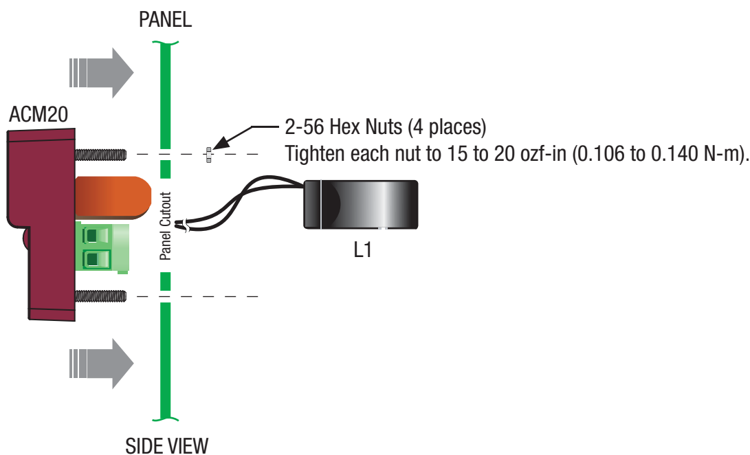
Figure 5. Panel Installation
