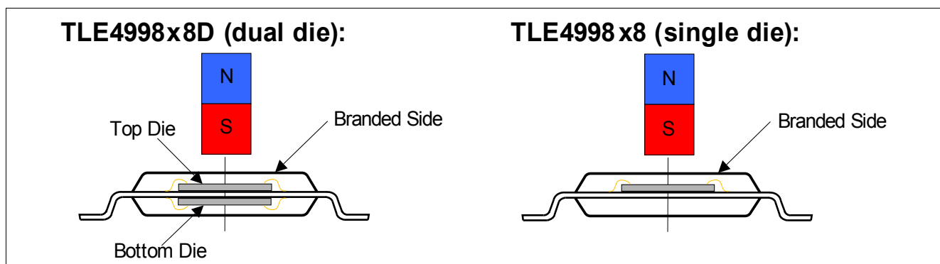
Figure 5-2 Definition of magnetic field direction of the TLE4998P8(D).
