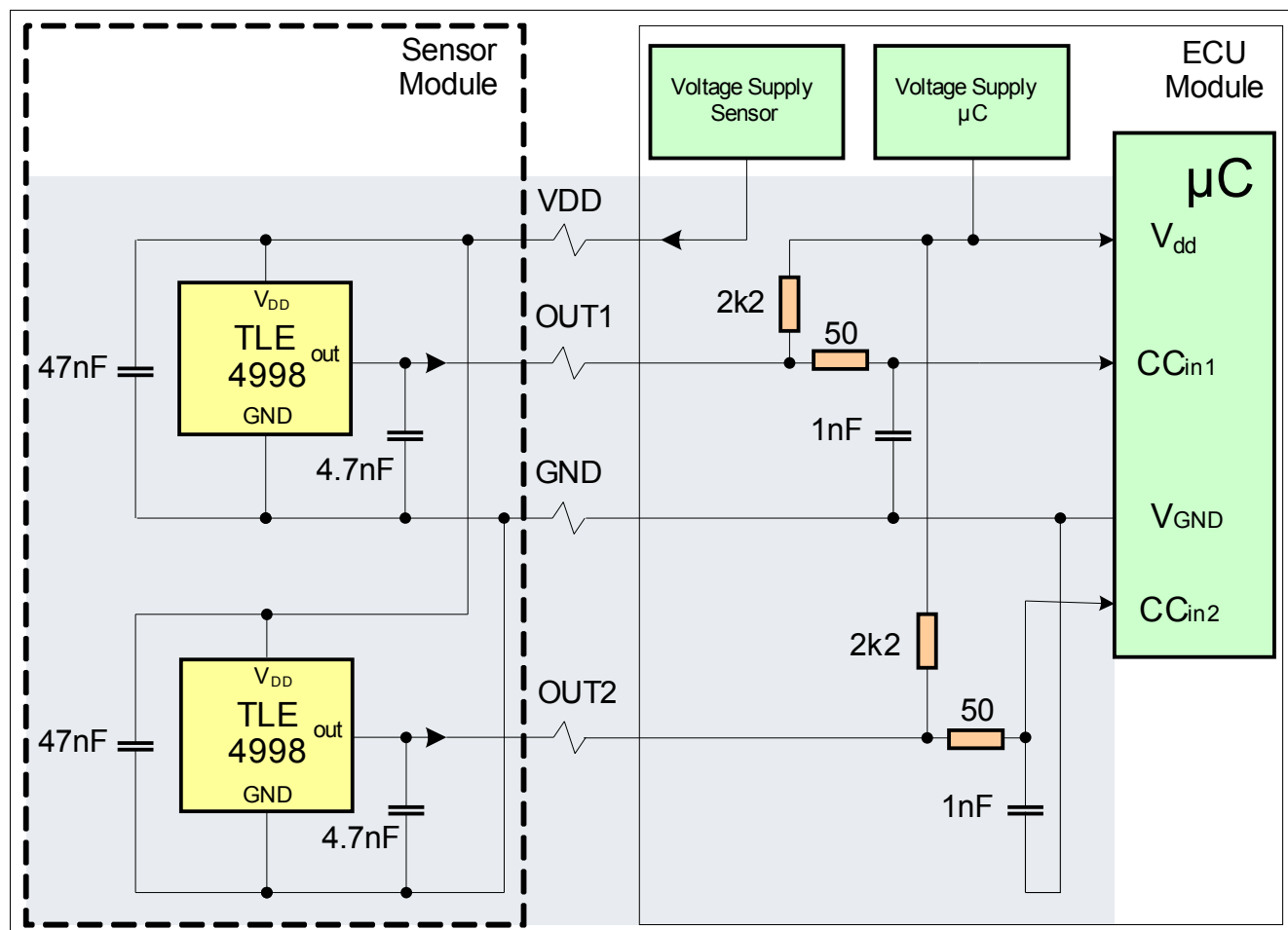
Figure 6-1 Application Circuit
