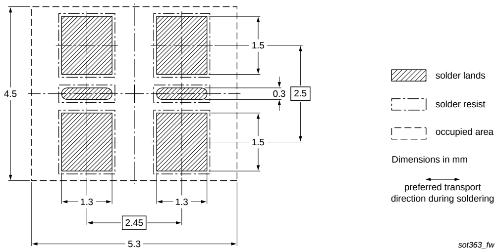
Fig 14. Wave soldering footprint PUMB10 (SOT363/SC-88)
