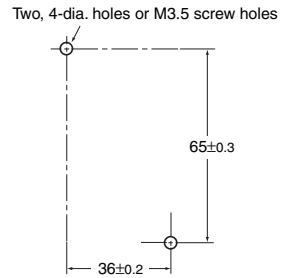
Mounting Holes (Top View)
