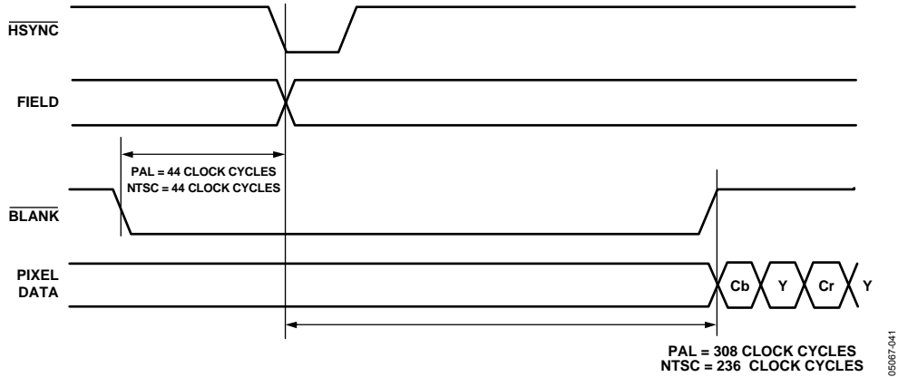
Figure 65. Active Pixel Timing
