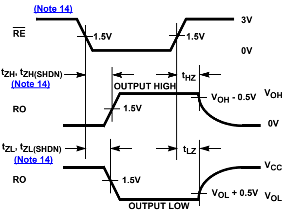
FIGURE 9B. MEASUREMENT POINTS
