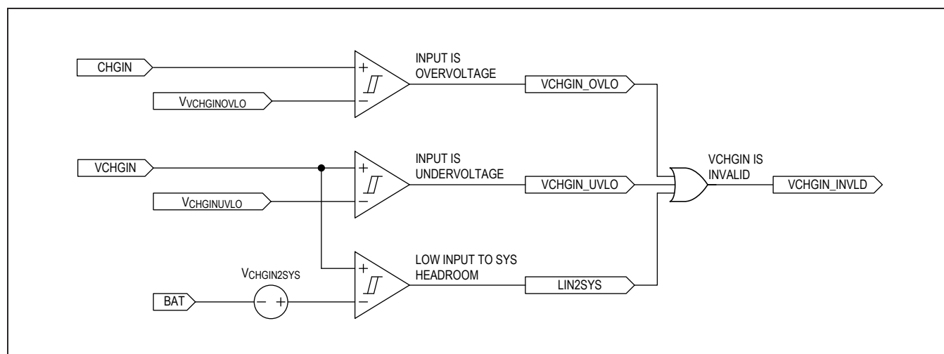
Figure 4. Charger Input Validation
