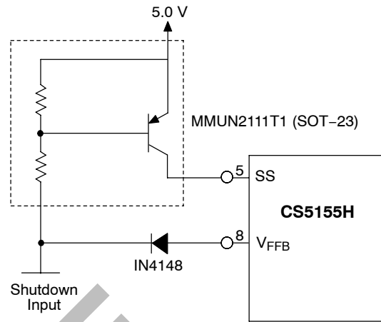
Figure 16. Implementing Shutdown with the CS5155H
