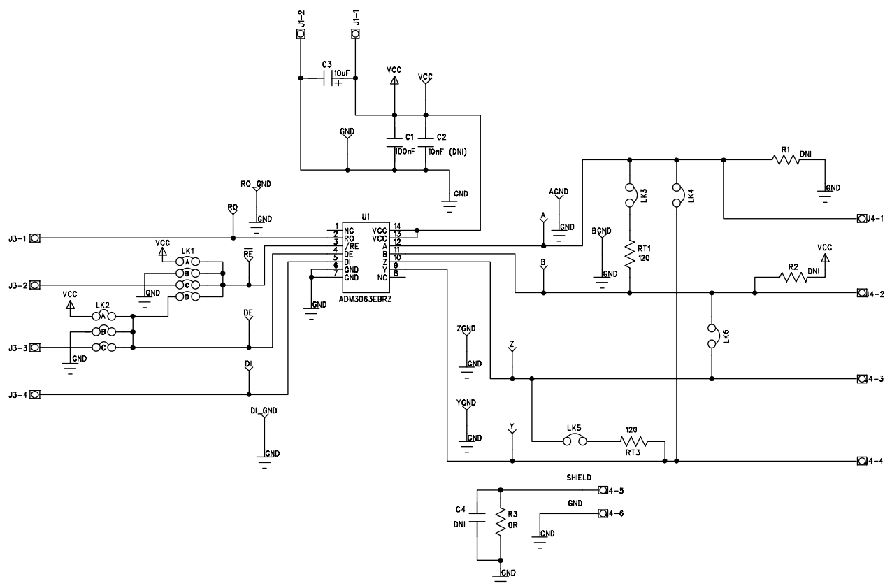
Figure 4. EVAL-ADM3063EEBZ Schematic
