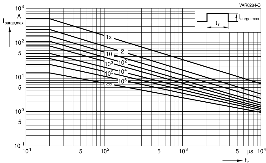
CT1812K35G ... K40G
