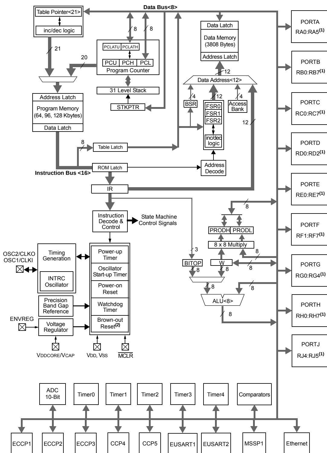
FIGURE 1-2: PIC18F86J60/86J65/87J60 (80-PIN) BLOCK DIAGRAM
