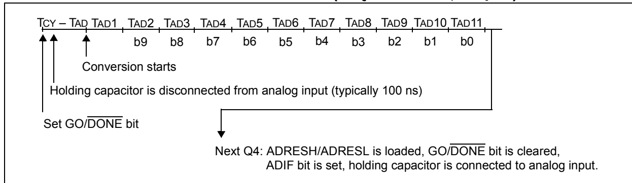
FIGURE 22-3: A/D CONVERSION \text{TAD} CYCLES ( \text{ACQT}<2:0> = 000 , \text{TACQ} = 0 )
