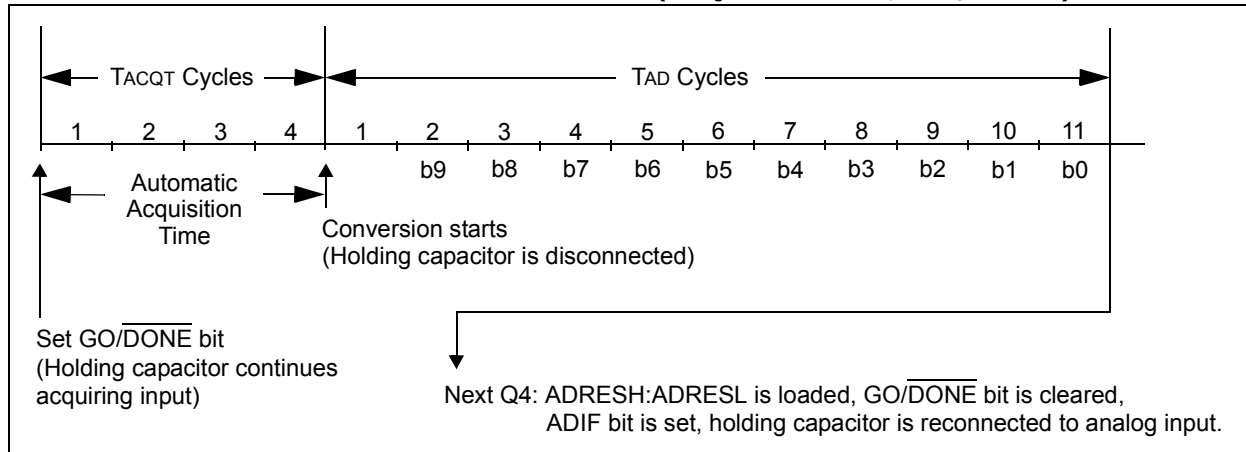
FIGURE 22-4: A/D CONVERSION \text{TAD} CYCLES ( \text{ACQT}<2:0> = 010 , \text{TACQ} = 4 \text{ TAD} )
