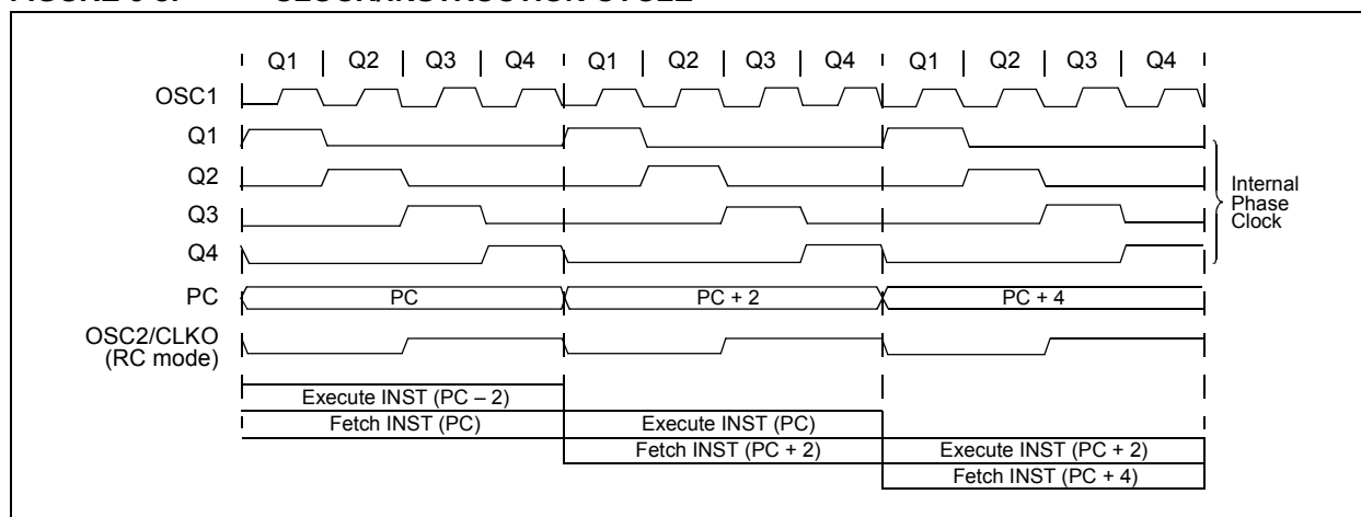
FIGURE 6-5: CLOCK/INSTRUCTION CYCLE
