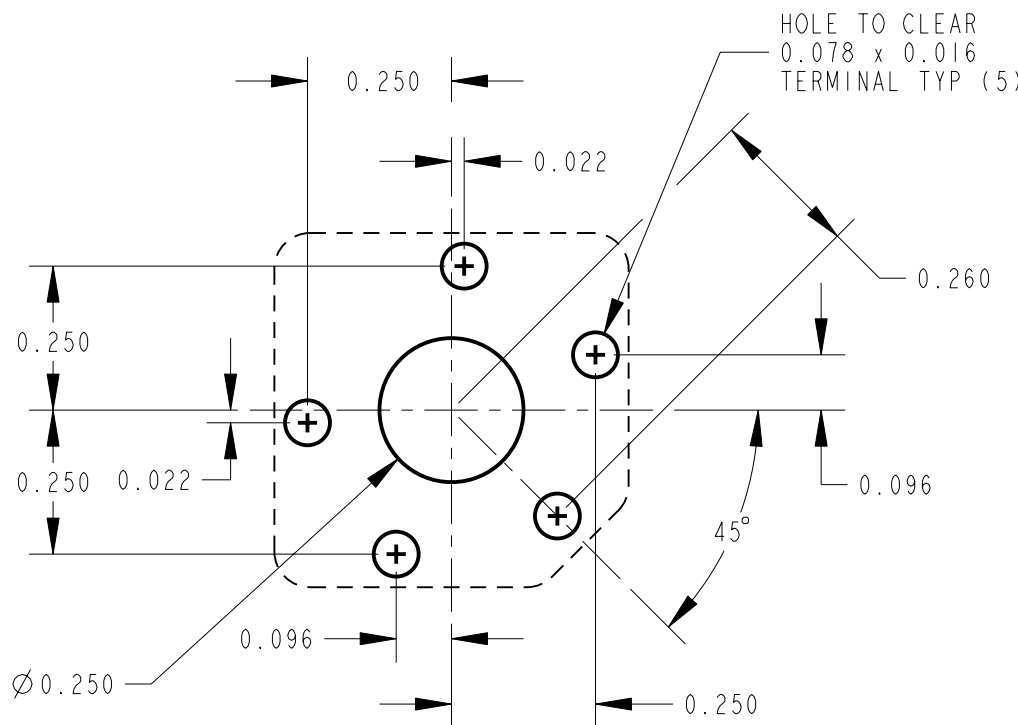
PC TERMINAL OPTION PCB LAYOUT - COMPONENT SIDE
