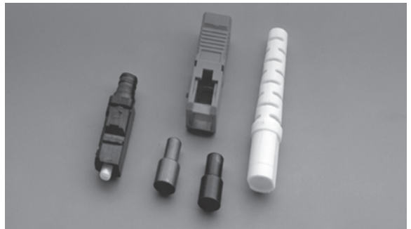
3M™ Crimplok™ SC Connector Single-mode
