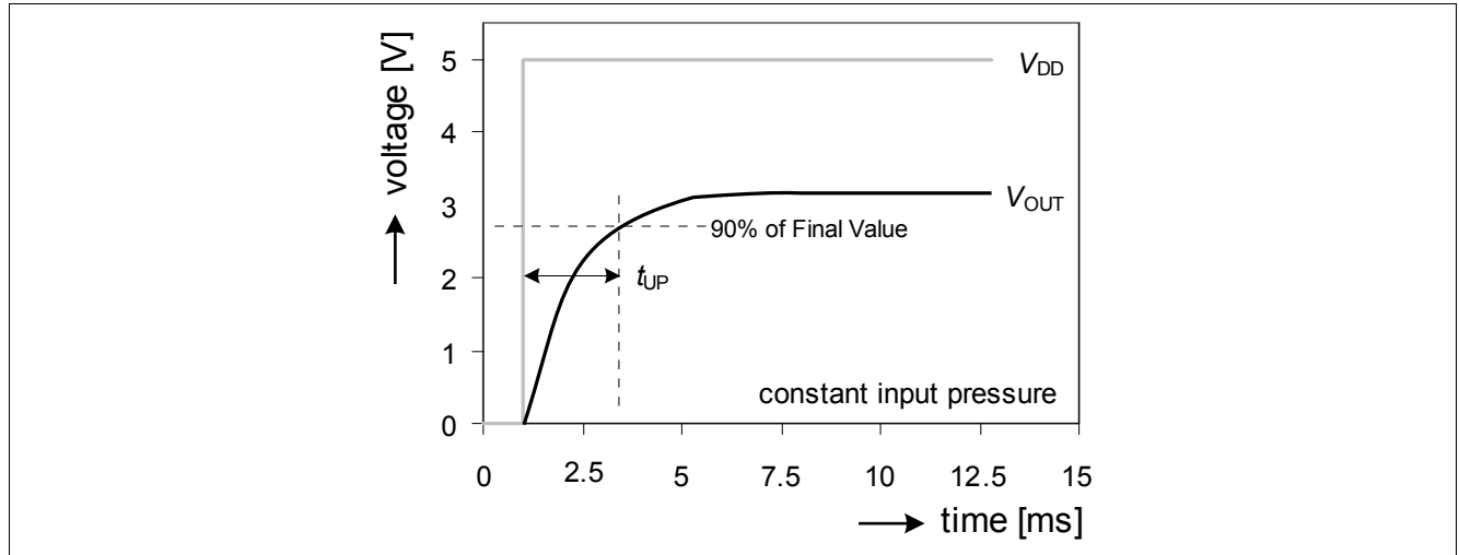
Figure 8 Power-up time
