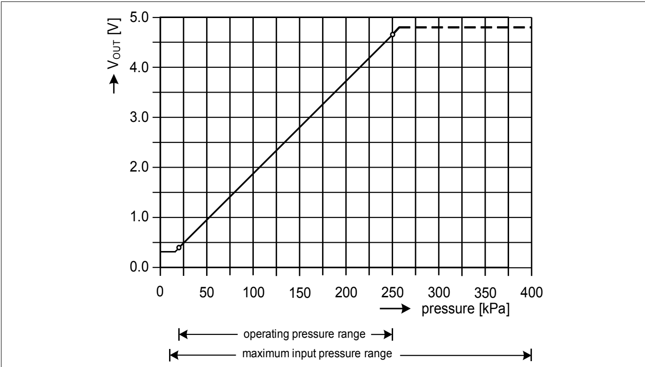
Figure 3 Transfer function
