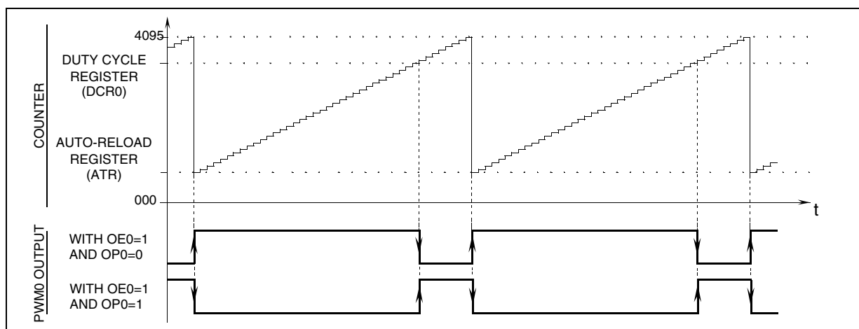
Figure 35. PWM Function
