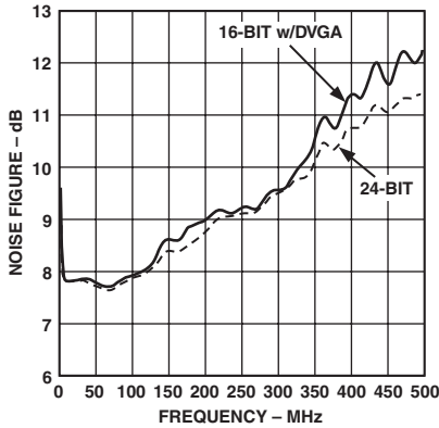
TPC 13a. Noise Figure vs. Frequency (Minimum Attenuation, f_{CLK} = 18\text{ MSPS} , BW = 10\text{ kHz} , High Bias)
