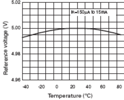
Temperature Drift
