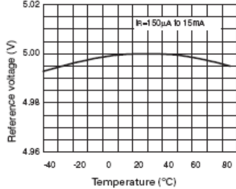
Temperature Drift
