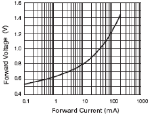
Forward Characteristics
