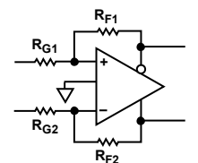
Figure 67. Typical Four-Resistor Feedback Circuit
