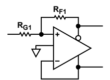
Figure 69. Typical Circuit with \beta_2 = 1
