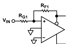
Figure 71. Typical Circuit with \beta_2 = 0
