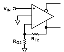
Figure 68. Typical Circuit with \beta_1 = 0
