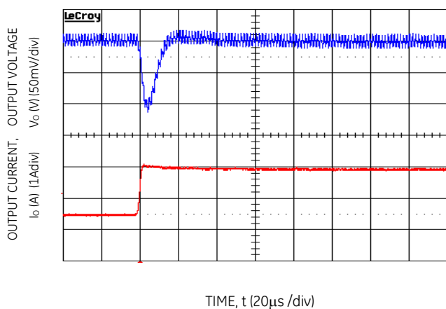
Figure 34. Transient Response to Dynamic Load Change from 50% to 100% at 12Vin, C_{out}=1\mu\text{F} , C_{Tune}=820\text{pF} & R_{Tune}=261
