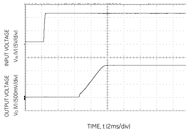
Figure 12. Typical Start-up Using Input Voltage ( V_{IN}=12\text{V} , I_o=I_{o,max} ).
