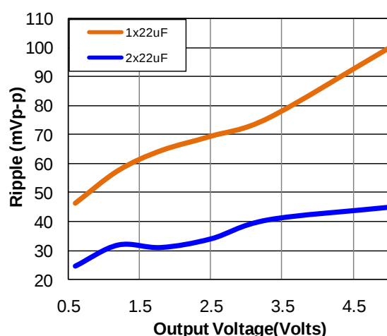
Figure 37. Input ripple voltage for various output voltages with 1x22 \mu F or 2x22 \mu F ceramic capacitors at the input (3A load). Input voltage is 12V.
