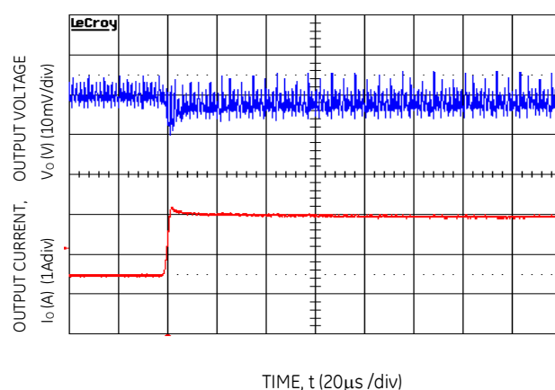
Figure 4. Transient Response to Dynamic Load Change from 50% to 100% at 8V in , C_{out}=1\times 47\mu\text{F}+2\times 330\mu\text{F} , C_{Tune}=27\text{nF} , R_{Tune}=178
