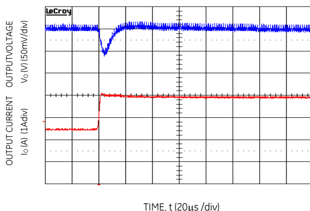
Figure 28. Transient Response to Dynamic Load Change from 50% to 100% at 12V in , C_{out}=2\times 47\mu\text{F} , C_{Tune}=2200\text{pF} & R_{Tune}=261
