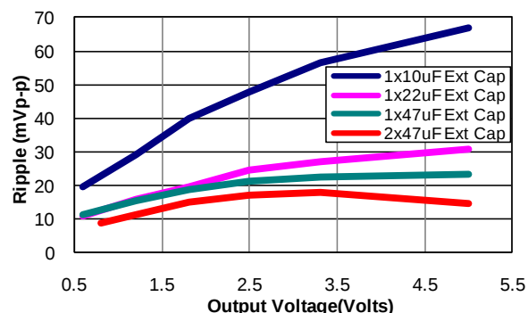
Figure 38. Output ripple voltage for various output voltages with external 1x10 \mu F, 1x22 \mu F, 1x47 \mu F and 2x47 \mu F ceramic capacitors at the output (3A load). Input voltage is 12V.
