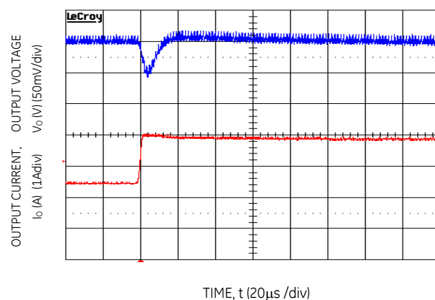
Figure 22. Transient Response to Dynamic Load Change from 50% to 100% at 12Vin, C_{out}=2\times 47\mu\text{F} , C_{Tune}=2700\text{pF} & R_{Tune}=261
