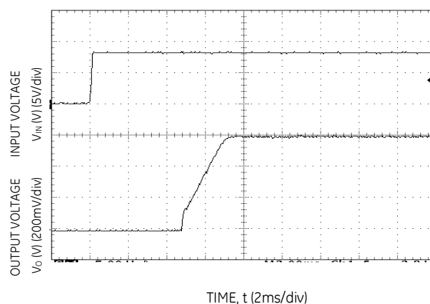
Figure 6. Typical Start-up Using Input Voltage ( V_{IN} = 8\text{V} , I_o = I_{o,max} ).
