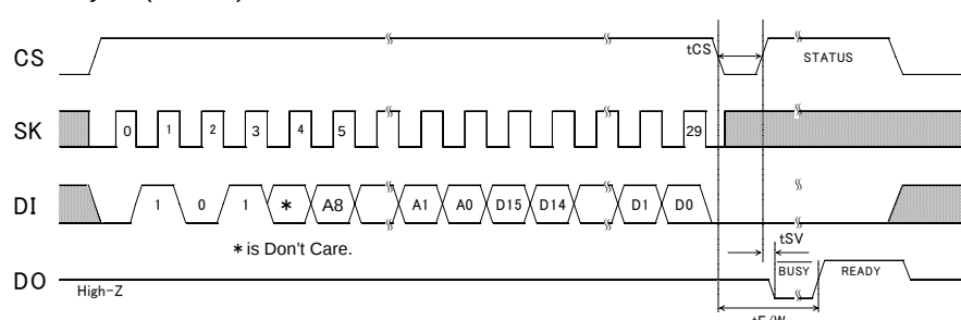
Figure 31. Write Cycle
