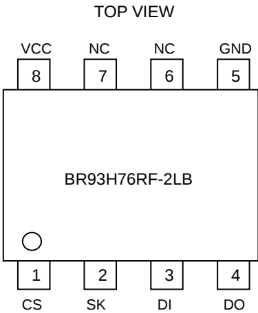
Figure 3. Pin Configuration
