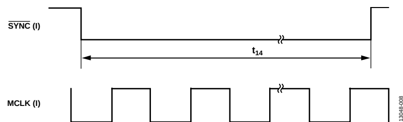
Figure 8. \overline{SYNC} Pulse Width
