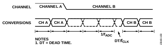
Figure 90. Sinc 3 Channel Change
