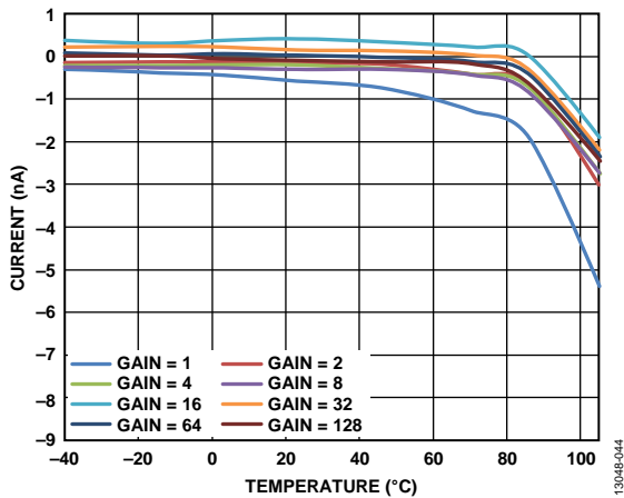
Figure 42. Absolute Analog Input Current vs. Temperature (Low Power Mode)
