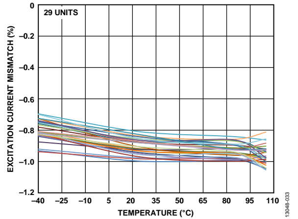
Figure 33. Excitation Current Drift Matching (500 µA)
