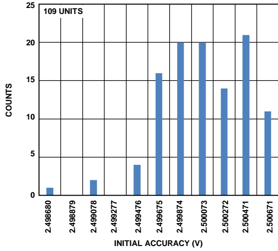
Figure 28. Internal Reference Voltage Histogram
