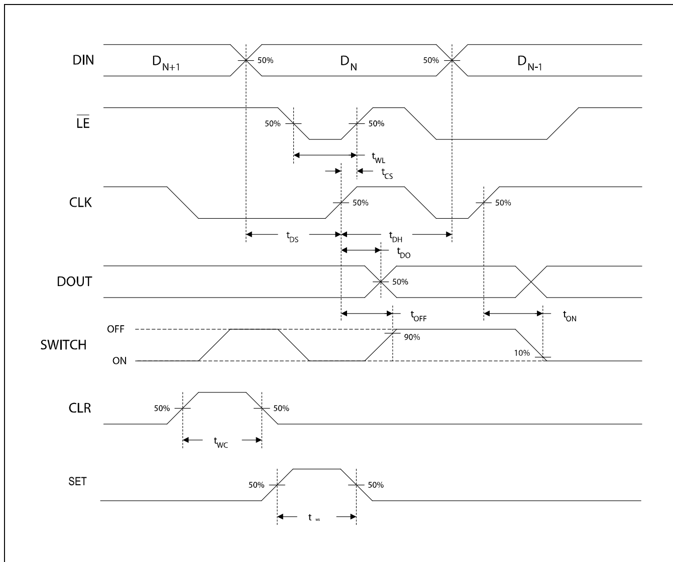
Figure 2. Timings
