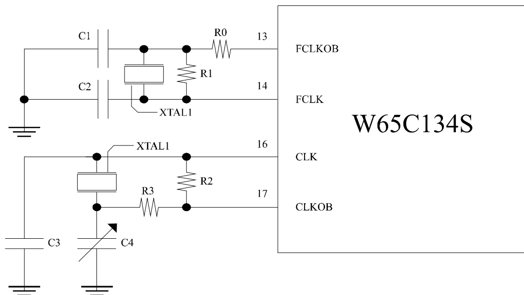
Figure 4-7 Oscillator Circuit
