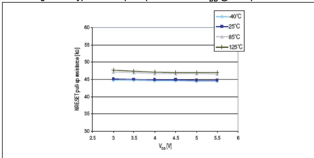
Figure 33. Typical NRST pull-up resistance vs V_{DD} @ 4 temperatures
