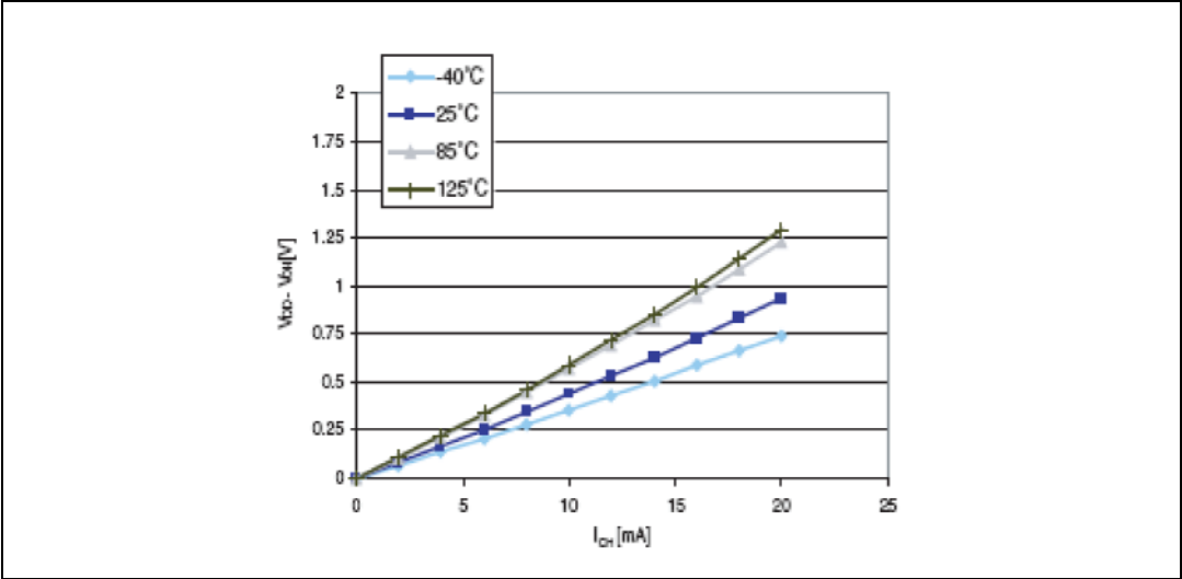
Figure 30. Typ. V_{DD} - V_{OH} @ V_{DD} = 5\text{ V} (high sink ports)
