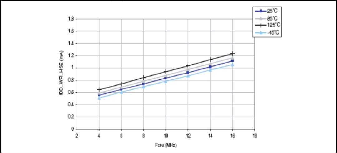
Figure 15. Typ I_{DD(WFI)} vs. f_{CPU} HSE user external clock, V_{DD} = 5\text{ V}
