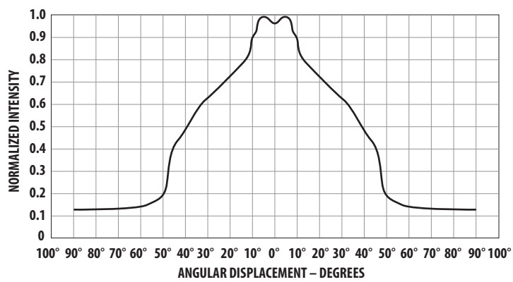
Figure 10. HLMP-P106/-P156.
