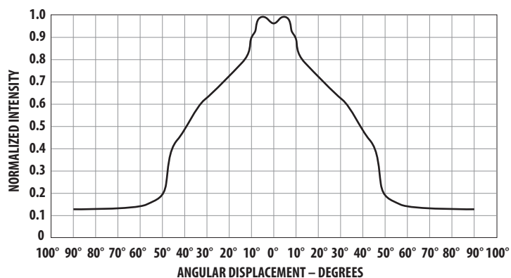
Figure 10. HLMP-P106/-P156.
