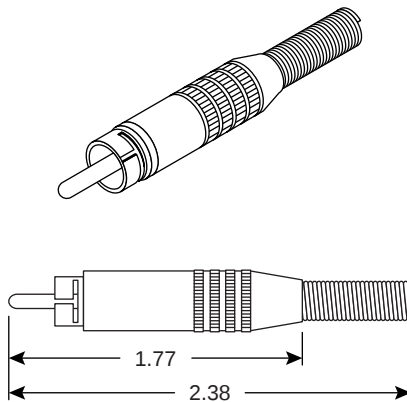
Dimensions (In.)
