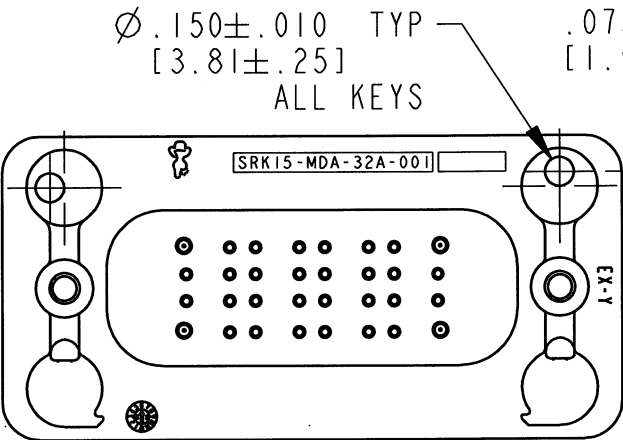
KEY ARRANGEMENT -A- SRK15-MDA-32A-001
