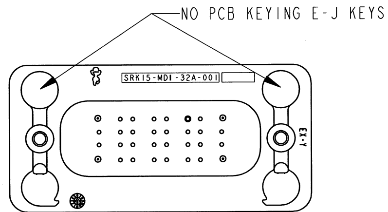
KEY ARRANGEMENT -I- SRK15-MDI-32A-001
