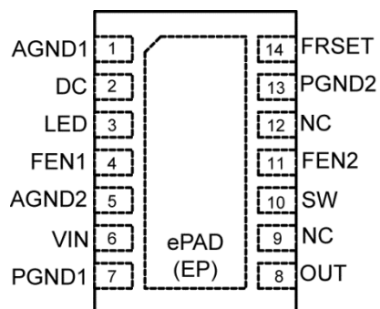
14-Pin 3mm × 2mm LDFN (MK) (Top View)
