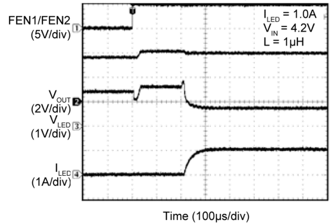
Flash Mode Turn-On Sequence (Linear Mode)
