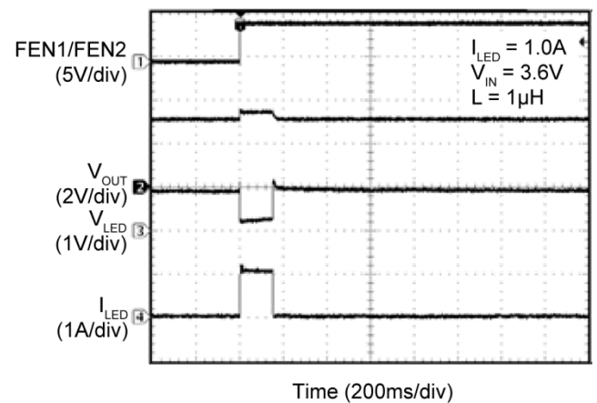
Flash Safety Timer at 150ms
