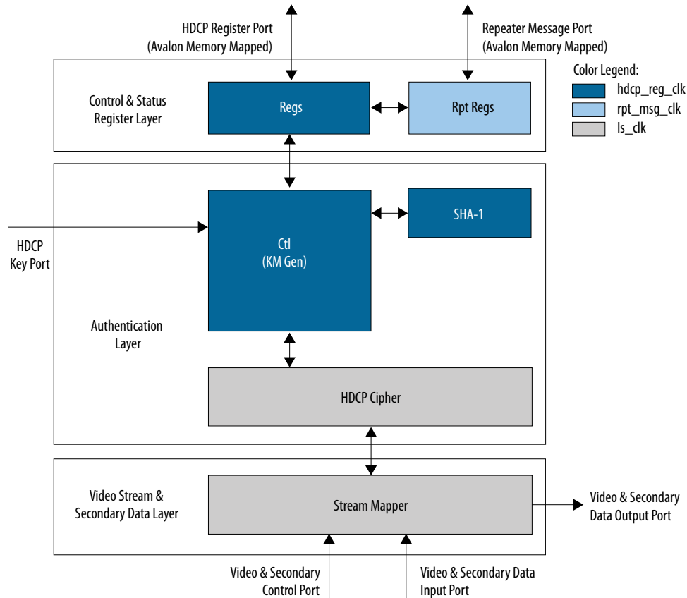
Figure 27. Architecture Block Diagram of HDCP 1.3 RX IP
