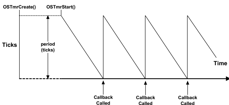
Figure 12-3 Periodic Timers ( dly == 0 , period > 0 )
