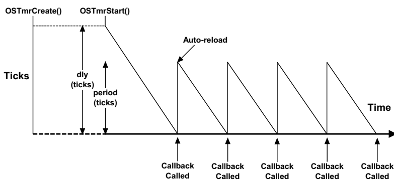
Figure 12-4 Periodic Timers ( dly > 0 , period > 0 )
