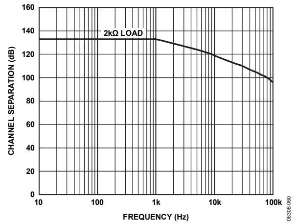
Figure 47. Channel Separation
