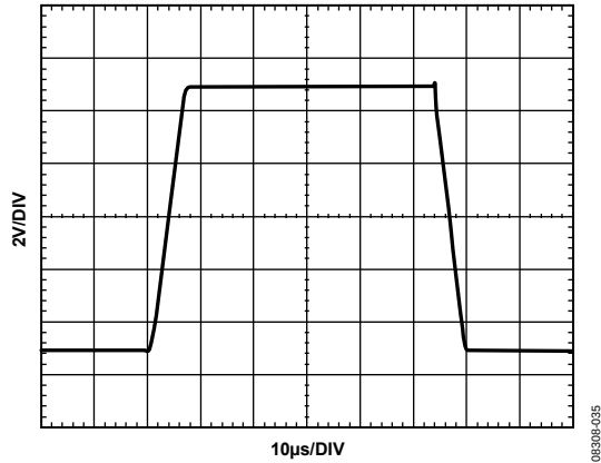
Figure 37. Large Signal Step Response, G = 1/2
