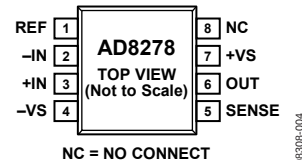
Figure 5. SOIC Pin Configuration
