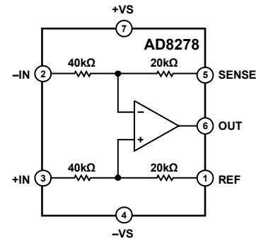
Figure 1. AD8278
