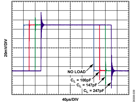
Figure 41. Small Signal Step Response for Various Capacitive Loads, G = 1/2
