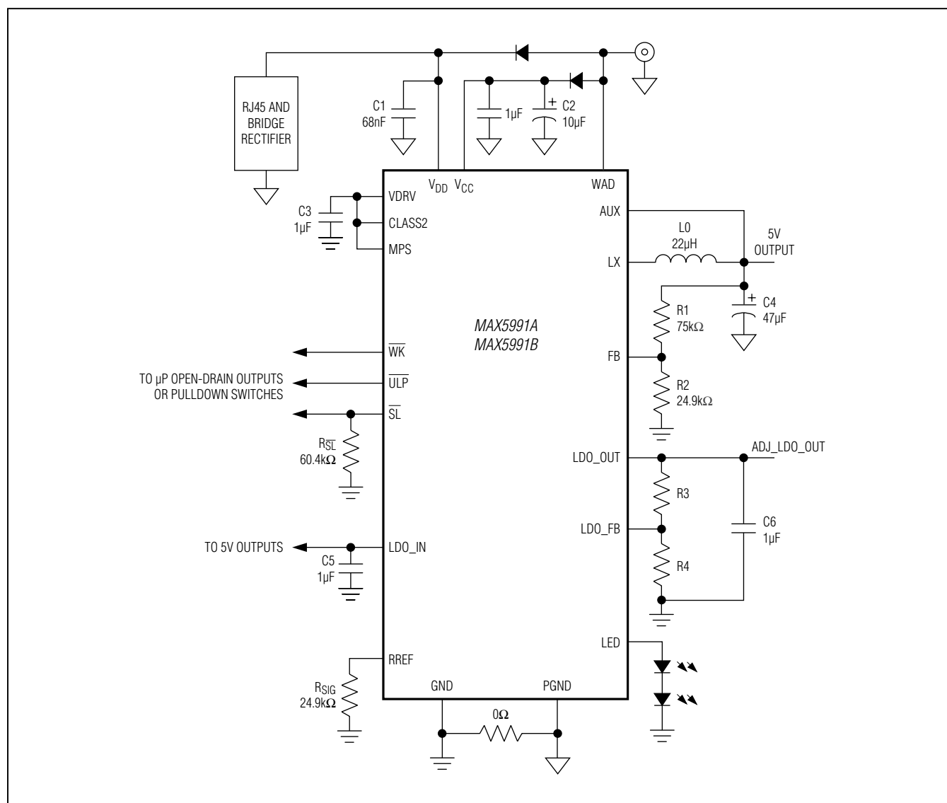
Figure 4. MAX5991A/MAX5991B 5V Buck Regulator and Adjustable LDO Output
