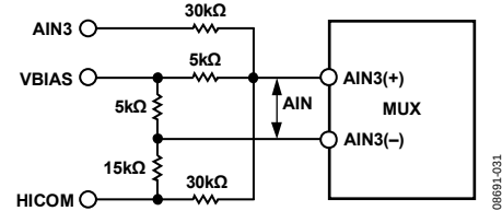
Figure 31. AIN3, High Level Input Channel Structure
