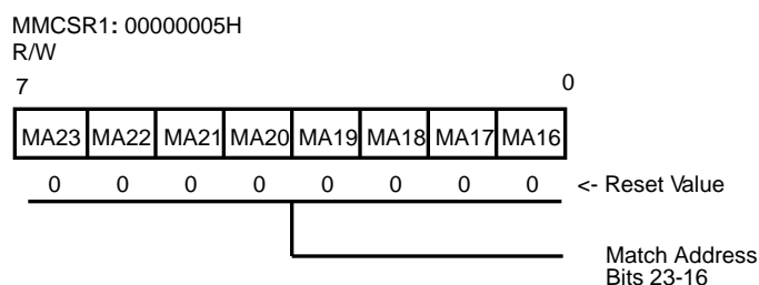
Figure 37. Mid-range Memory Chip Select Register 1
