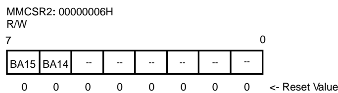
Figure 38. Mid-range Memory Chip Select Register 2
