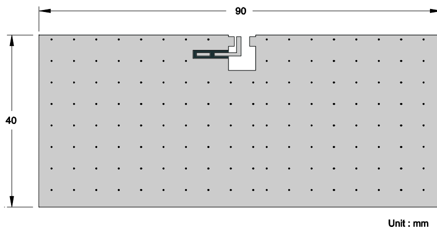
Fig. 3 Outlook and dimension of evaluation board
