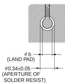
DETAIL OF \textcircled{C} PART
