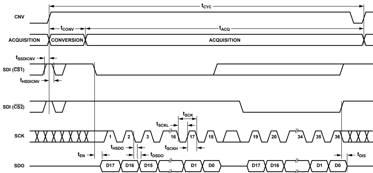
Figure 40. 4-Wire \overline{\text{CS}} Mode Without Busy Indicator Serial Interface Timing
