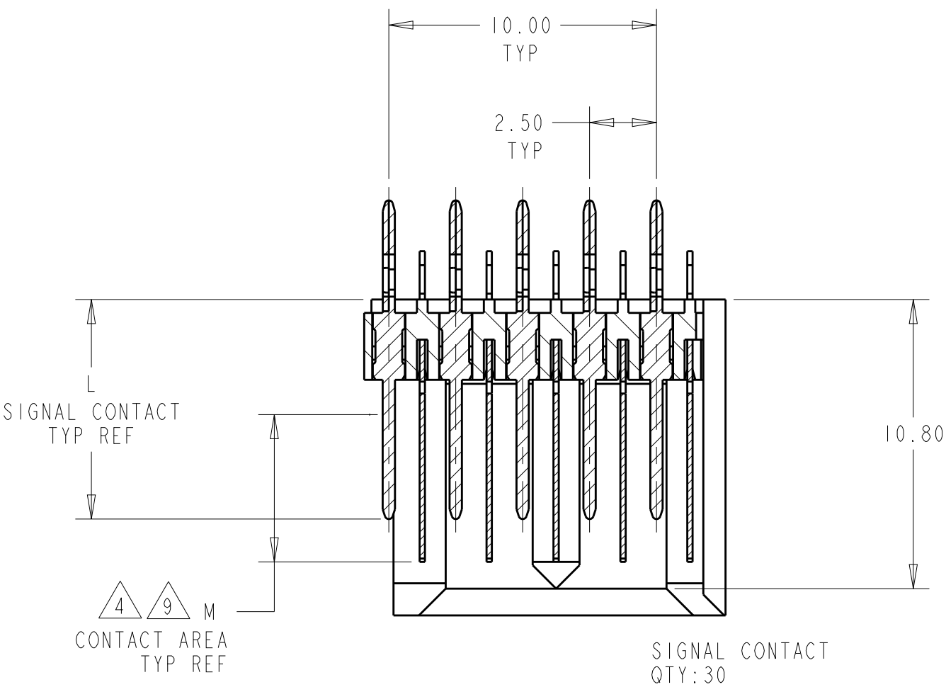
SECTION B-B
