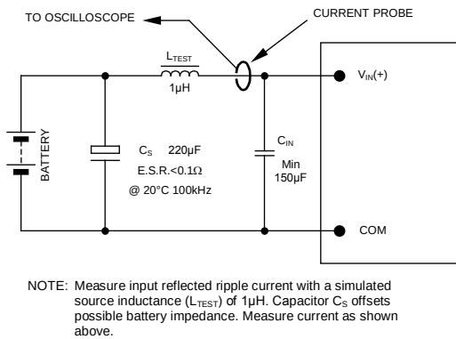
Figure 43. Input Reflected Ripple Current Test Setup.
