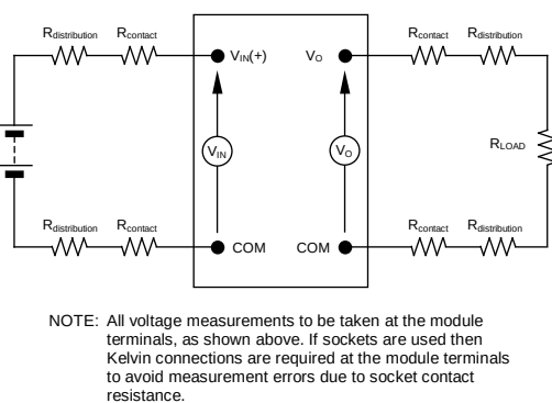
Figure 45. Output Voltage and Efficiency Test Setup.
