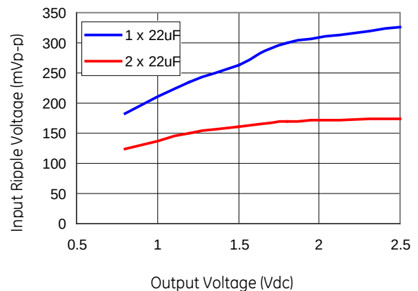
Figure 46. Input ripple voltage for various output voltages with 1x22 μF or 2x22 μF ceramic capacitors at the input (30A load). Input voltage is 12V.
