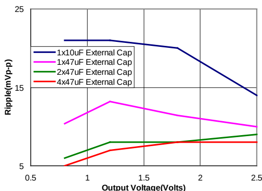
Figure 49. Output ripple voltage for various output voltages with external 1x10 \mu\text{F} , 1x47 \mu\text{F} , 2x47 \mu\text{F} or 4x47 \mu\text{F}
