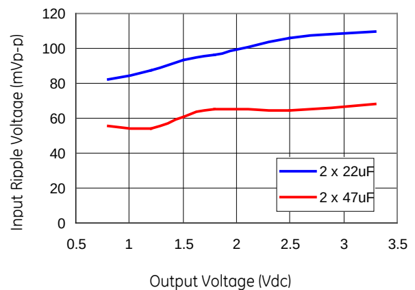
Figure 47. Input ripple voltage in mV, p-p for various output voltages with 2x22 μF or 2x47 μF ceramic capacitors at the input (30A load). Input voltage is 5V.
