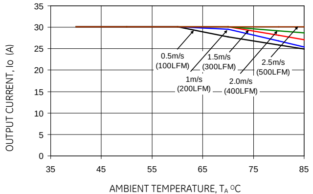
Figure 28. Derating Output Current versus Ambient Temperature and Airflow (ATS030A0X3-SRH).
