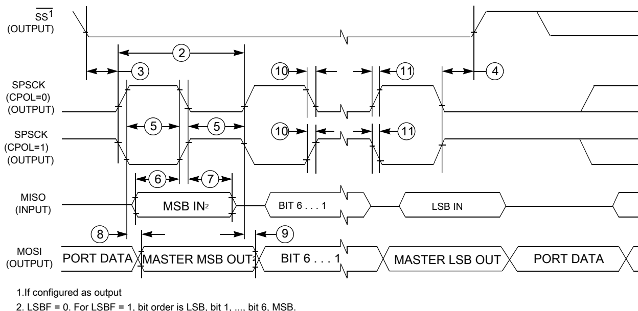
Figure 14. SPI master mode timing (CPHA = 1)
