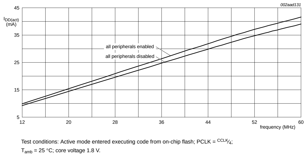
Fig 9. Typical LPC2119/01 and LPC2129/01 I_{DD(act)} measured at different frequencies
