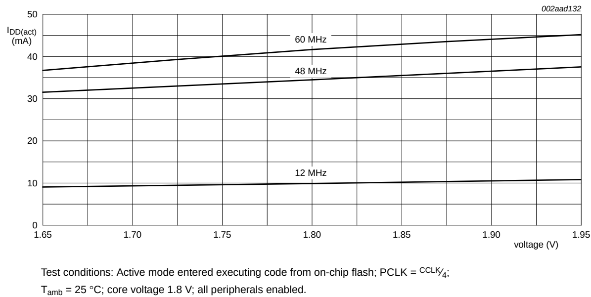
Fig 10. Typical LPC2119/01 and LPC2129/01 I_{DD(act)} measured at different voltages
